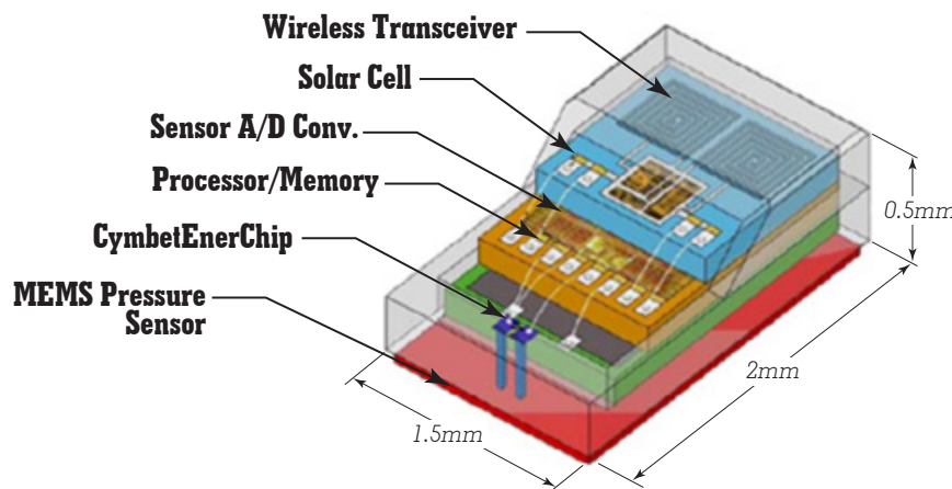
Figure 3: IOPM Layers Block Diagram.
