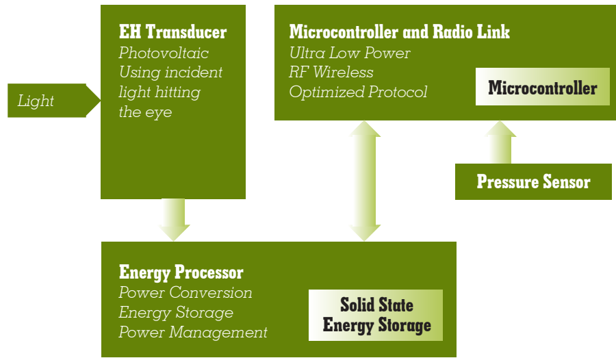
Figure 2: IOPM Wireless Sensor Block Diagram.
